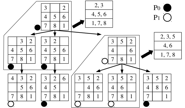
Figure 2: Distribution of nodes according to Abstract Zobrist hashing on 2 threads, using a projection from a cell to a row of the puzzle. States inside the lines are assigned to the same processor because they share the same abstract features.
